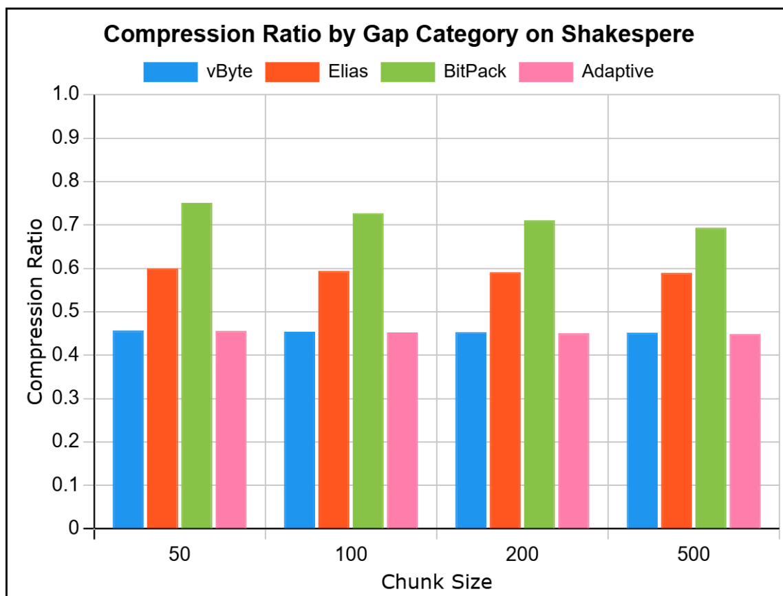
Figure 1. Compression ratio size by chuck size for each compression method
